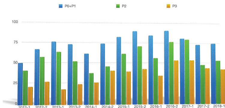
Completeness per priority in percent
