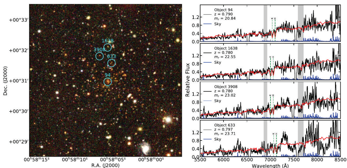
Left: 5'x5' false-colour optical image of the z = 0.79 cluster ACT-CL J0058.1+0031. SALT spectra for four galaxies (cyan circles) are shown to the right. Black lines: smoothed SALT/RSS spectra; red lines: best match redshifted SDSS spectral template; blue line: sky spectrum; gray bands: regions strongly affected by absorption features in the atmosphere.
