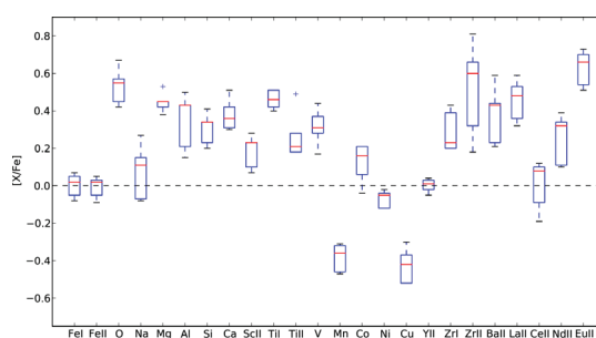
Abundance pattern for the sample of RGB stars in NGC 6584. The boxes represent the inter-quartile range (i.e., the middle 50% of the sample), while the red horizontal line in each box denotes the median value. Outliers beyond 1.5 times the second and third quartile are indicated as blue crosses.
