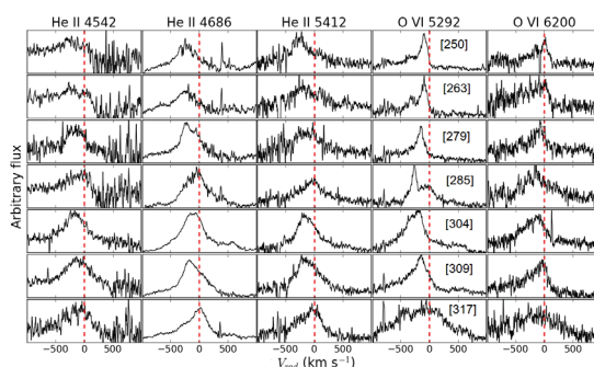
The evolution of the profiles of the 'moderately narrow' emission lines (labelled at the top) of V407 Lup. A heliocentric correction was applied to the radial velocities. The flux is in arbitrary units. The numbers in brackets are days since discovery. The red dashed lines represent the rest-wavelength of each line ( v_{\text{rad}} = 0 km/s).
