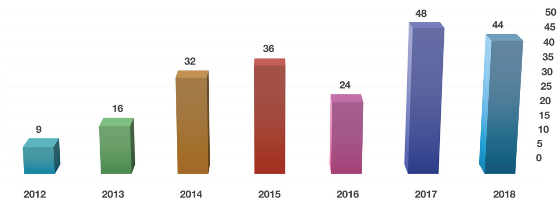
Refereed papers based on SALT science data (i.e., excluding instrument-related publications), from 2012 onwards.
