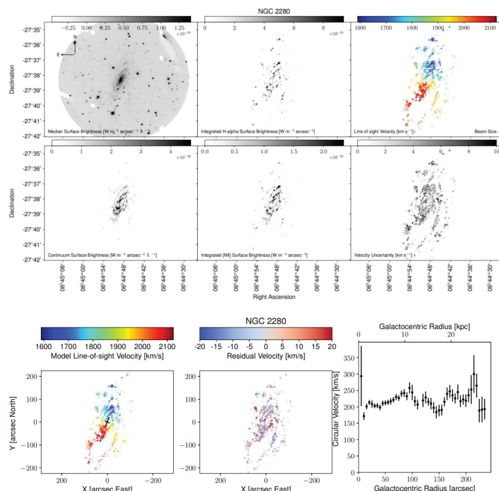
SALT observations and models of NGC 2280. Shown are the median R -band surface brightness, continuum surface brightness, H \alpha surface brightness, N II surface brightness, line-of-sight velocity, velocity uncertainty, DiskFit kinematic model, model residual, and extracted rotation curve.
