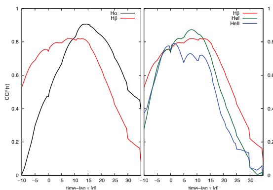
Fig 3: CCFs of the integrated H \alpha , H \beta , He I \lambda 5876, and He II \lambda 4686 lines with respect to the continuum at 4570 Å.
