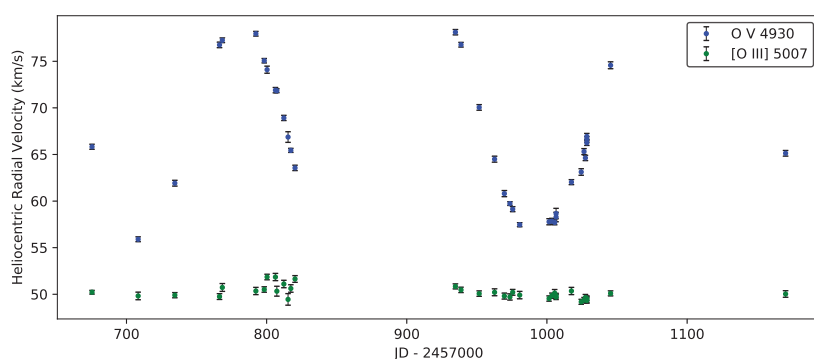
SALT/HRS radial velocity measurements of the central star of NGC 1360 using the O V \lambda 4930 stellar emission line (blue). The radial velocity of the nebular O III \lambda 5007 emission line is shown for comparison (green). Note the clear 142 d periodic variability in the central star due to orbital motion.
