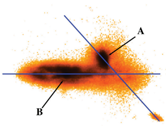
Left: SDSS r -band image of the merger J1100+1002 showing the RSS slit positions. The strong radio emission is associated with the nucleus of galaxy A.
