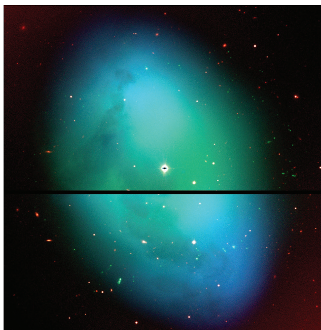
ESO VLT-FORS2 colour-composite image of NGC 1360 made from images taken with I -band (red), H \alpha +N II (green) and O III (blue) filters.
