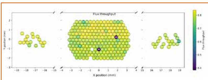
Flux throughput for the SMI-300 fibres.
