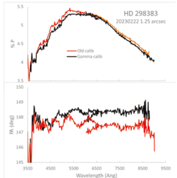
Figure 1: Comparison of old and new calibration for HD 298383, using a narrow slit.
