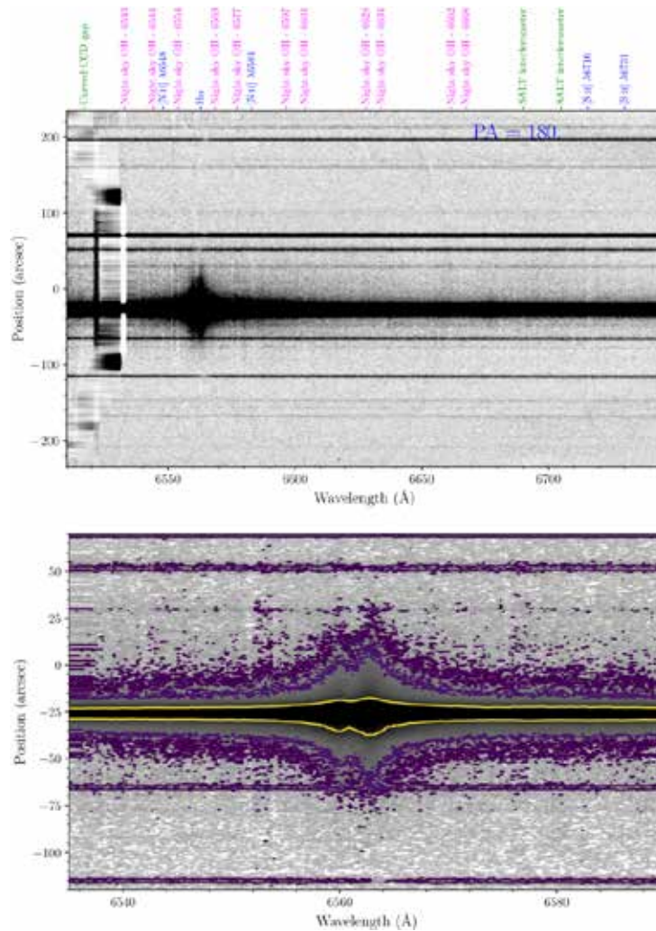
Top: Sky-subtracted SALT spectrum of the inner RS Oph shell. All unidentified (vertical) lines are due to the night sky. Unidentified horizontal lines are field stars that were aligned with the slit during the observations. Bottom: A close-up of the sky-subtracted region around H \alpha . The black, grey, and purple pixels are, respectively, at least 200, 20, and 2 counts above background.
