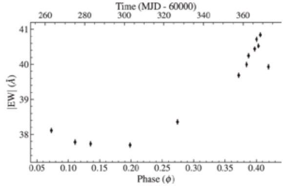
Orbital modulation of the H \alpha equivalent width as measured with SALT.
