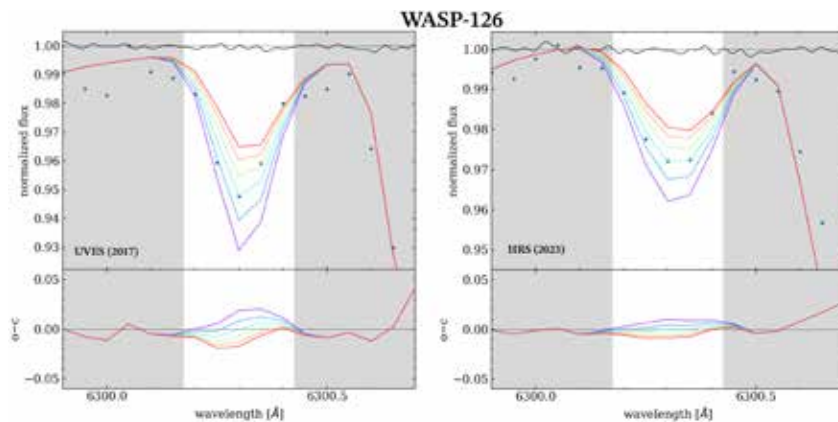
The [O I] line at 6300 Å in spectra from VLT/UVES (left) and SALT/HRS (right). The observed spectra are marked with blue dots in the upper panels; coloured lines are the synthetic spectra for different O abundances, separated by 0.1 dex; the black solid line represents the telluric spectrum. The rms of the residuals (lower panel) is 0.0014 and 0.0005 for UVES and HRS, respectively.
