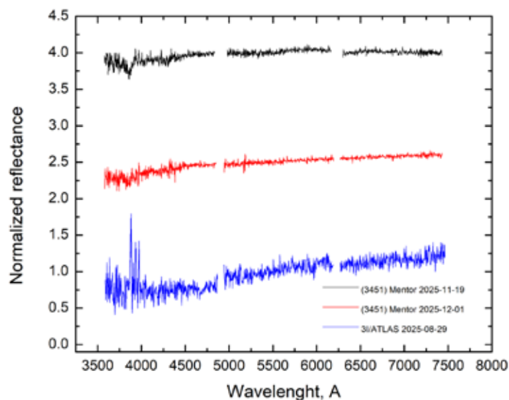
Black and red curves: reflectance spectra (spectra of the asteroid divided by a spectrum of the solar analogue star) of asteroid (3451) Mentor from observations on 2025-11-19 and 2025-12-01. No activity was detected during either visit. Blue curve: reflectance spectrum of the active object 3I/ATLAS, obtained on 2025-08-29, showing strong CN emission at 3880 Å, consistent with a cometary classification. All spectra were obtained using RSS with grating PG0700 at R \sim 1800 .
