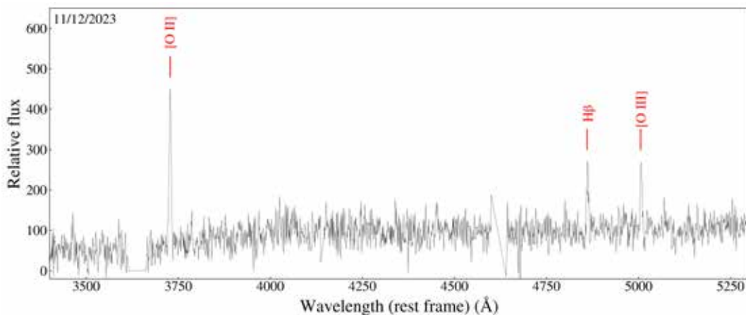
A SALT spectrum showing several emission lines which enabled the redshift calculation.
