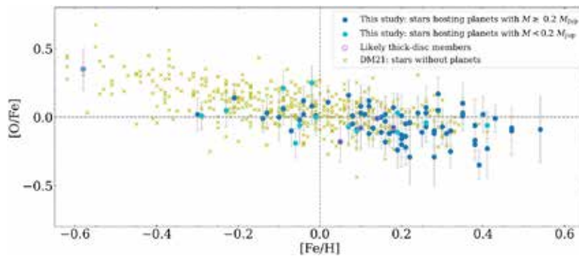
[O/Fe] abundance ratios as a function of the stellar metallicity. Light and dark blue points refer to planet-hosting stars. Yellow crosses are for single stars without planets
