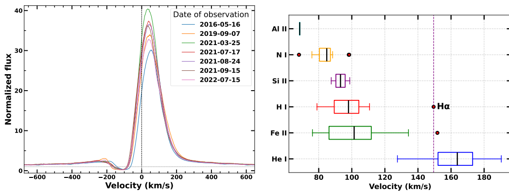
Left: Variability of the H \alpha line from seven epochs of SALT data. Right: The box plot of velocities of various species identified in SALT spectra.
