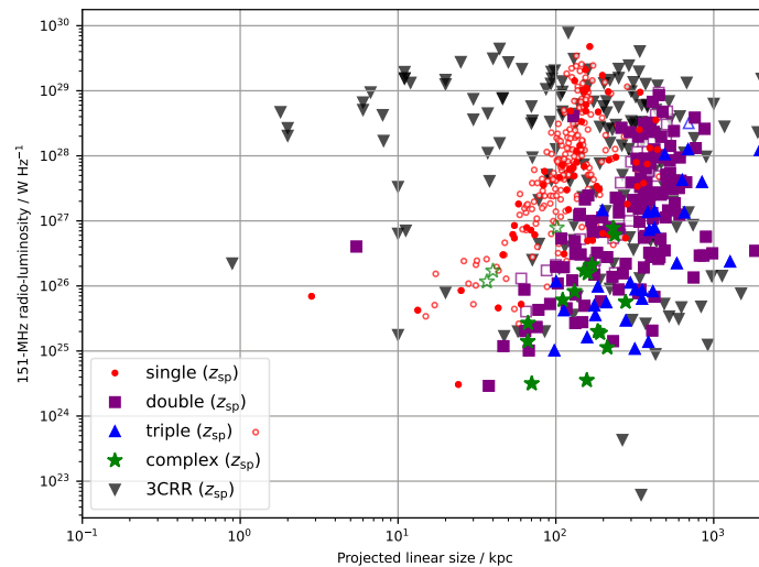
The radio-power–size (P–D) diagram for the G 4 Jy sample, as a function of radio morphology. Upper limits in the linear size are represented by unfilled symbols. Spectroscopic redshifts ( z_{sp} ) are from SALT and other telescopes.
