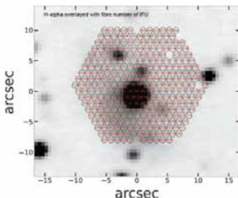
Left: H \alpha image from SALTICAM of SXP 31.0 showing the halo. Right: The same overlaid with the fibre IFU positions.
