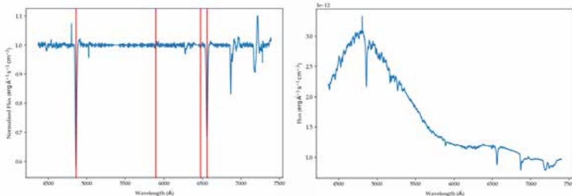
Example spectrum before and after being flattened ( left and right , respectively).
