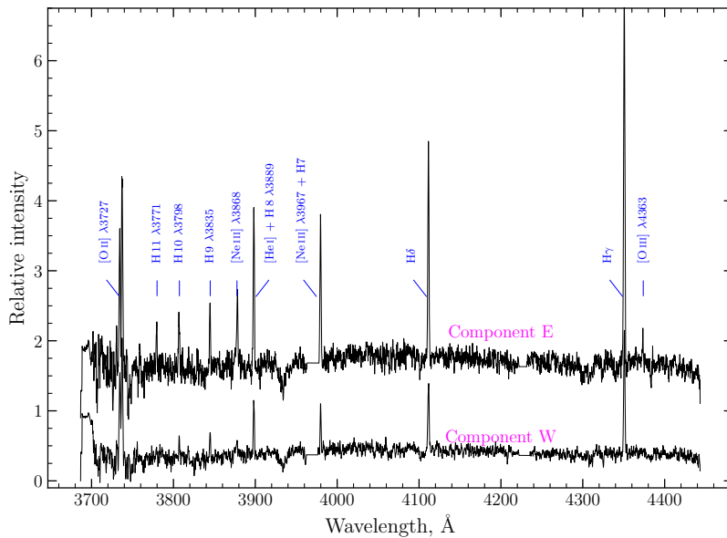
Top: HST image of the Peekaboo galaxy, resolved into stars, with the position of SALT’s slit superimposed. The bluest massive stars and compact blue nebulae are marked with numbers. Bottom: Spectra of two [H II] regions with emission lines indicated. In component E, the auroral line of the oxygen ion [O III] λ4363, used in the direct method of determining the metallicity of gas, is clearly visible.
