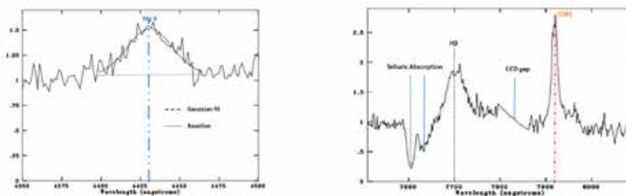
Annotated spectral emission lines of the AGN LMC1SNE5. The spectrum shows that [MgII] \lambda 2798 is detected in the blue setting (left) and [OIII] \lambda 5007 is detected in the red setting (right). The redshift of the source is 0.582 \pm 0.001 . H \beta is also detected but cut on the blue side by telluric absorption at 7600 Å; likewise, H \gamma is detected but cut (on the red side) by telluric absorption. The CCD gap fell just between H \beta and [OIII]. A Gaussian was fit to the [MgII] line.
