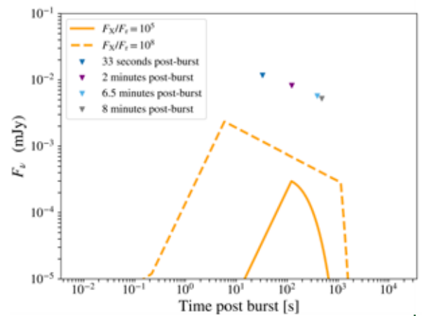
A comparison of the upper flux limits to the synchrotron maser model.
