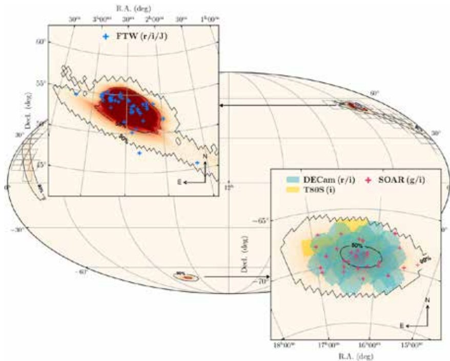
Localisation region of S250206dm overlapped with the footprints of GW-MMADS follow-up observations. The upper and lower inset panels show zoomed-in views of two lobes of the LVK sky map with high probability, located in the northern and southern hemispheres, respectively. For reference, the grey outline indicates the sky tiles in the northern lobe used for ZTF observations of S250206dm.
