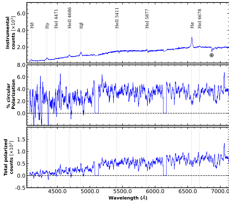
The spectra of 1RXS J080114.6–462324 obtained on 21 January 2025, centred at the spin phase \phi = 0.816 . Prominent emission lines are indicated, while the \oplus symbol marks regions affected by atmospheric telluric features. From top to bottom, the panels present the average spectrum, the circular polarisation percentage spectrum, and the total polarised flux.
