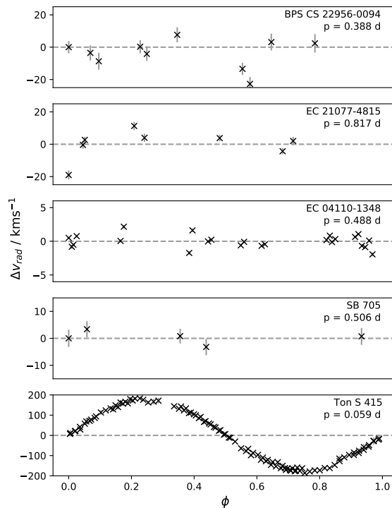
Radial velocity measurements from cross-correlation for the SALT candidate binaries. Each star's measurements have been phase-folded to their periods. Apart from Ton S 415, no candidates show significant radial velocity variations corresponding to their photometric periods. The formal error in each RV measurement is shown in grey.
