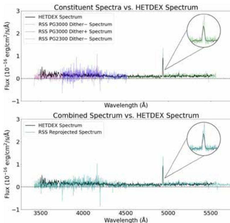
Target spectrum flux density (black line) from the HETDEX catalogue plotted against wavelength. Top : the spectrum of each observation (grating) overlaid on HETDEX; bottom : the aggregated extracted spectrum post wavelength reprojection. The zoom-in insets on the [O II] region show the successful resolution of the doublet and accurate wavelength calibration. The continua and emission line flux for this target matched HETDEX to well within 20% error.
