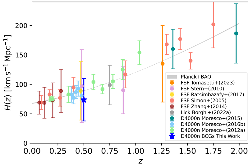
H(z) derived from the cosmic chronometers method at different redshifts. The team’s estimate using only BCGs is shown with a blue star at z = 0.5 . Labels refer to measurements made using full-spectrum fitting (FSF), Lick indices, or D4000_n . For reference, the standard \Lambda CDM Planck evolution is shown in a grey band with its width determined by \pm 1\sigma variation of cosmological parameters.
