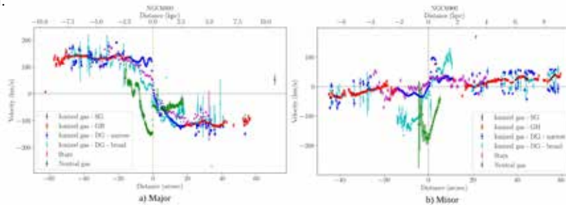
Rotation curves of NGC 6000 with RSS long-slit spectra along the major (a) and minor (b) axes. The black dashed lines indicate the optical photometric centre of the galaxy and the velocity associated with it. The dashed orange line indicates the kinematic centre. The velocities of the ionised gas is shown in blue (narrow) and cyan (broad) points for the double Gaussian (DG) model, red plus signs for the Gaussian-Hermite (GH) model and black crosses for the single Gaussian (SG) model. The velocities of the neutral gas are shown as green diamonds, and the velocities of the stars are shown as magenta points. The rotation curves suggest an ionised and neutral gas outflow from the centre of the galaxy as well as the disc.
