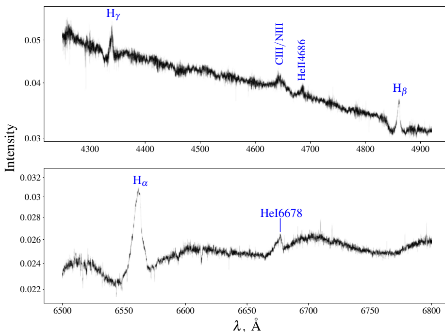
Blue ( top ) and red ( bottom ) arms of J161201's SALT/HRS spectrum. The HRS provides data in arbitrary, uncalibrated intensity units. Identified emission lines are labeled.
