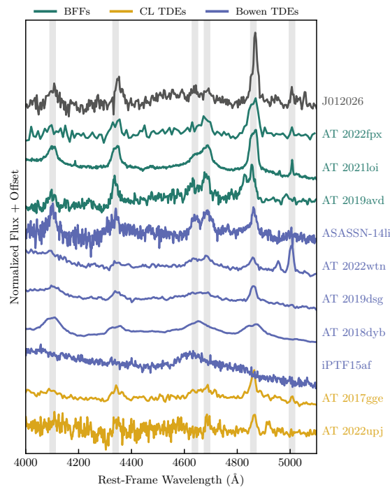
Comparison of optical spectra of J012026 with other members of the BFF class (green), TDEs with Bowen Lines (blue), and TDEs with coronal lines (CL TDEs, yellow). The grey shaded areas show, respectively from left to right, the wavelength corresponding to H \delta , H \gamma , [N III], [He III], H \beta and [O III] \lambda 5007. The spectrum of J012026 resembles more closely the spectra of BFFs.
